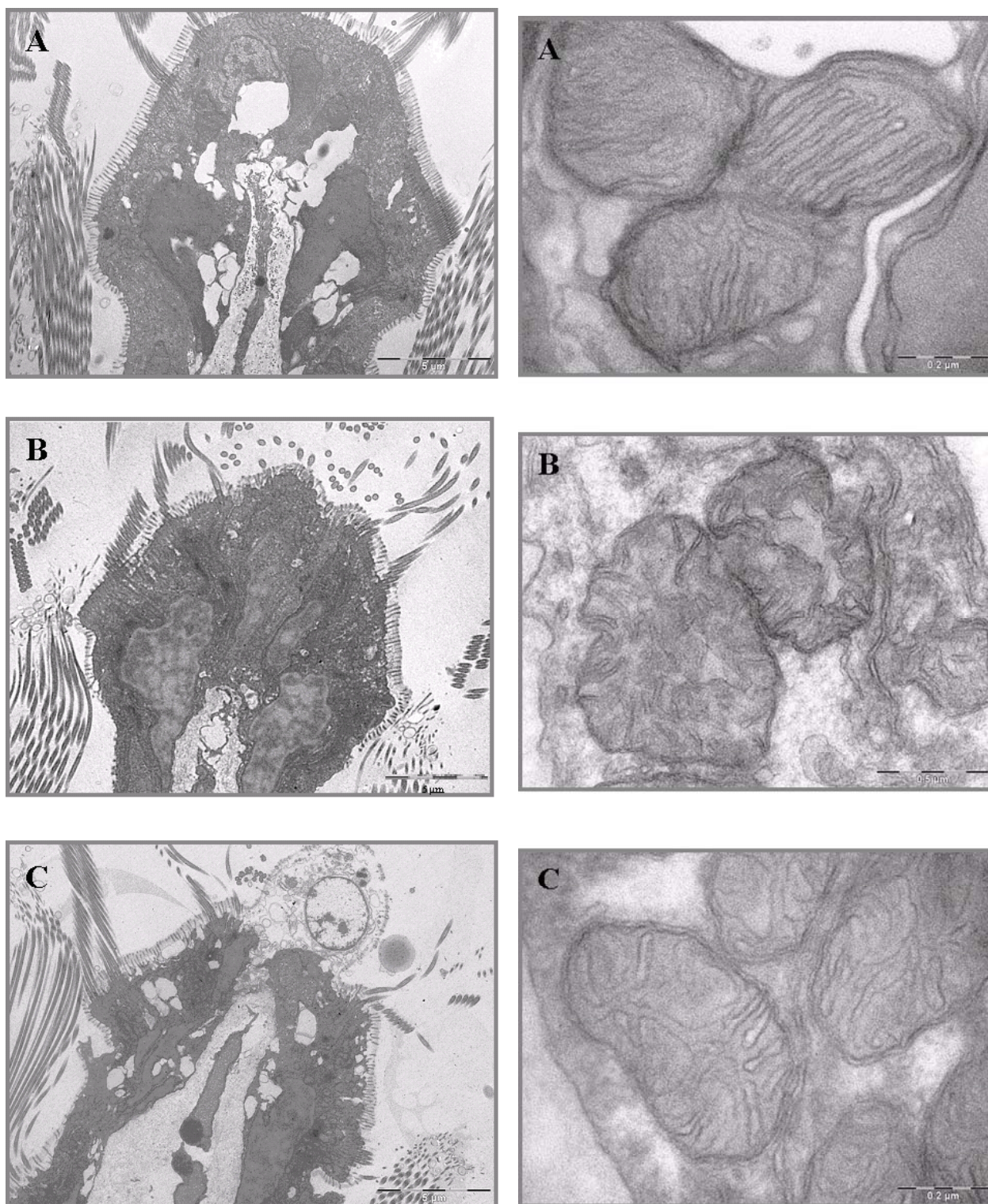
Figure 24 Influence of selenium on the gill ultrastructure of C. fluminea . A : control group ; B : group exposed to SeMet; C : group exposed to selenite. On the left side, the frontal zone of gill filaments is displayed. Vacuoles are observed in this zone for the control group and for selenite exposed group while for SeMet no vacuoles are seen. For the selenite exposed group, lots of apoptotic cells are observed in this frontal zone. On the right side, mitochondria in filament cells are presented. Mitochondria of SeMet exposed group appear with a dented outer membrane, cristae arranged irregularly and a matrix becoming more electron lucent.
