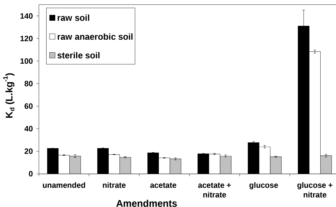
Figure 1 Distribution coefficients, K_d ( \text{L.kg}^{-1} ) for soil samples constrained to various microbiological states
