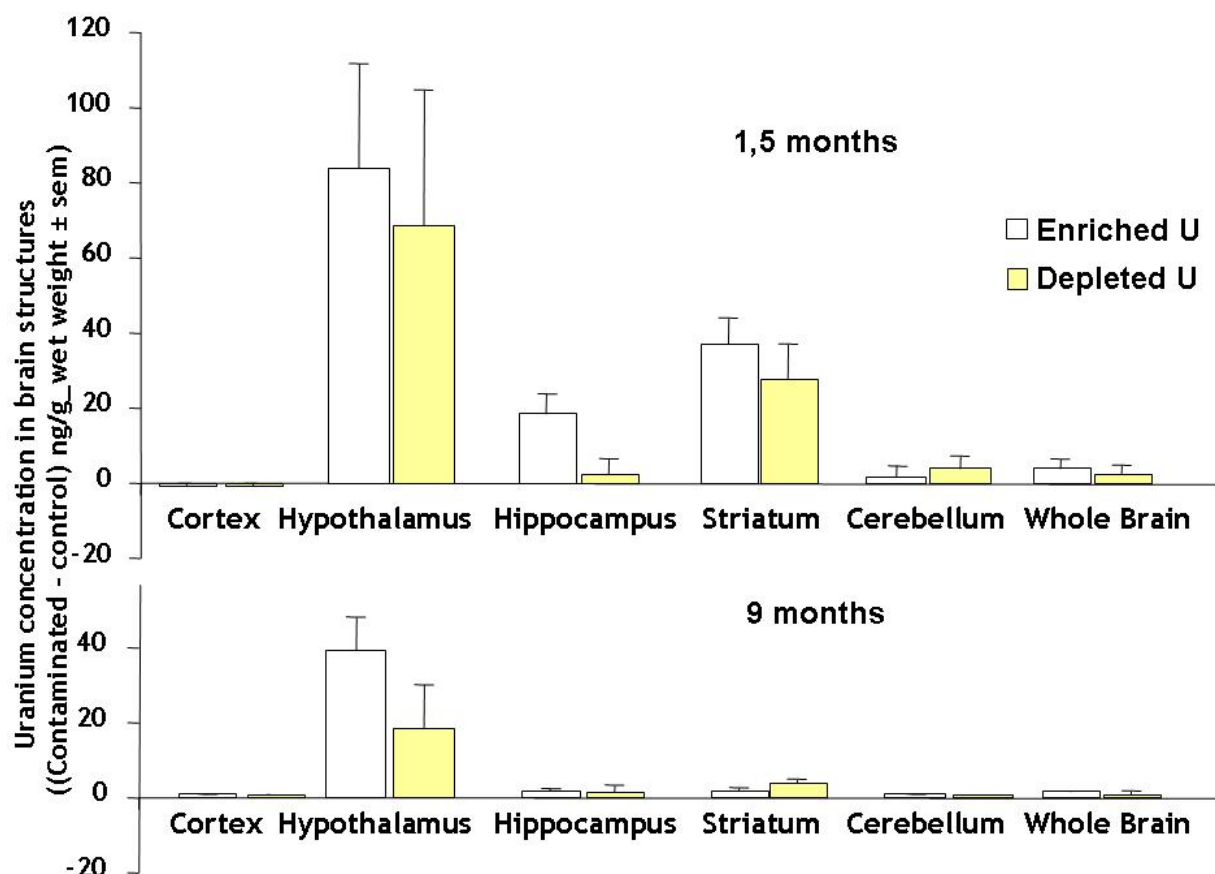
Figure 15 Uranium concentration in the main brain structures of exposed rats (ng/g_wet weight \pm sem). The values of control rats have been subtracted.
