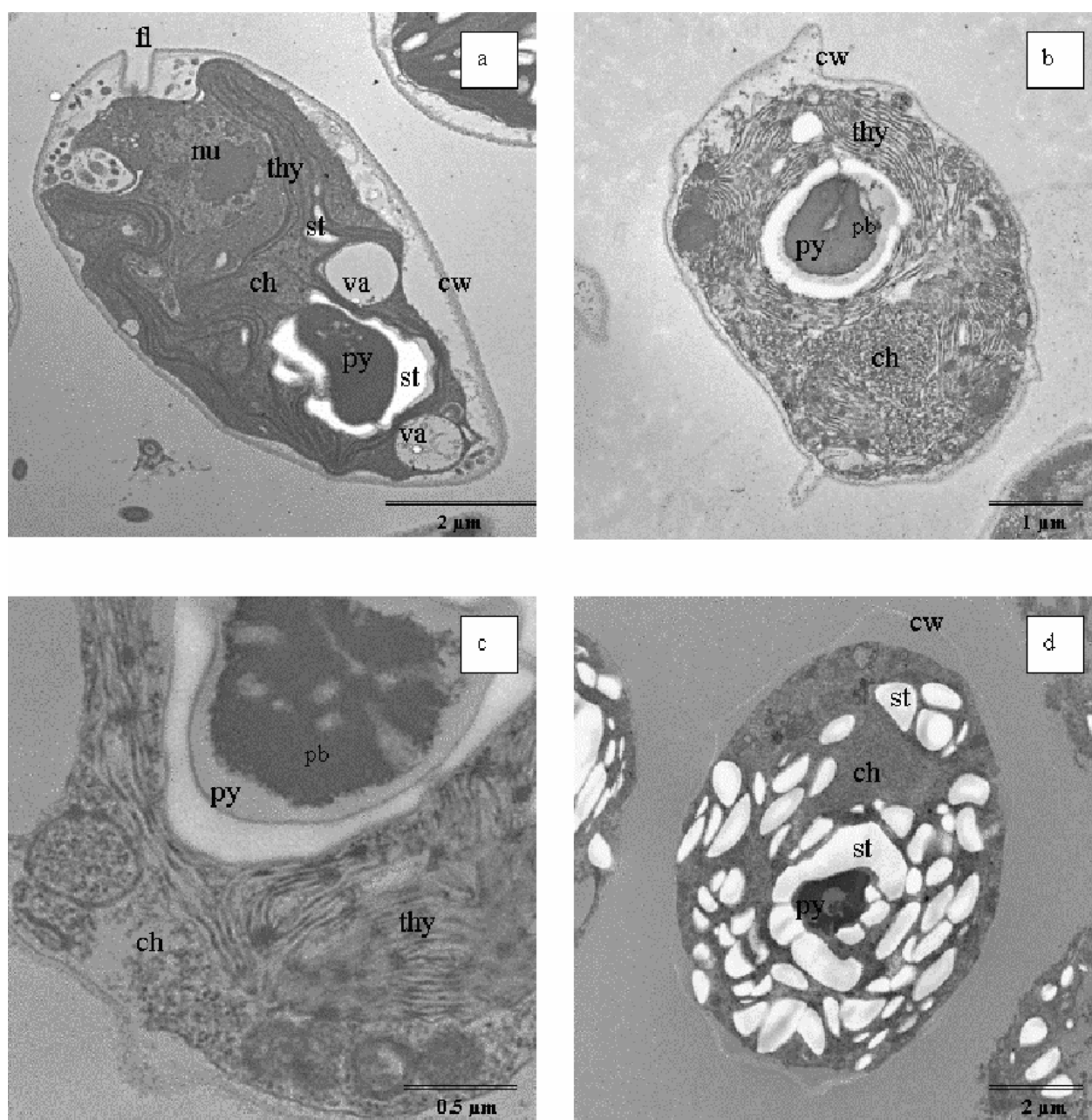
Figure 22 Influence of selenite on the ultrastructure of Chlamydomonas reinhardtii : detailed structures of cells harvested 96 hours after inoculation. a: control. The oval cells are enclosed within a rigid cell wall (cw) principally made of glycoproteins. Two pairs of flagella (fl) emerge from an apical depression. About 40% of the cell volume is taken up by the chloroplast (ch). This organelle consists of a double layered envelope, a stroma and mostly parallel layers of thylakoids (thy). Longitudinal cross sections typically show a U-shaped structure surrounding the nucleus (nu), with a broad basal area containing a prominent pyrenoid (py) (the protein body (pb) consists primarily of RUBISCO). Starch bodies (st) are present all around the pyrenoid and in the stroma. Controls contained a lot of empty vacuoles (va). b and c: 50µM. Thylakoids are of a fingerprint-like appearance and the pyrenoid shows signs of structural disintegration with partially dissolved protein bodies d: 500µM. Cells accumulate starch to a large extent, structures are severely disrupted and normal cell organelles are often indistinguishable.
