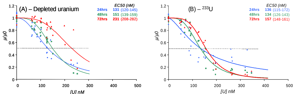
Figure 16 Effect of (A) depleted uranium and (B) 233 U on the growth inhibition of the green algae Chlamydomonas reinhardtii at pH=5, modified HSM medium. EC 50 are given with their 95% interval confidence (n=3 ; Regtox Fit with the Hill model and bootstrap simulation - n=500)
