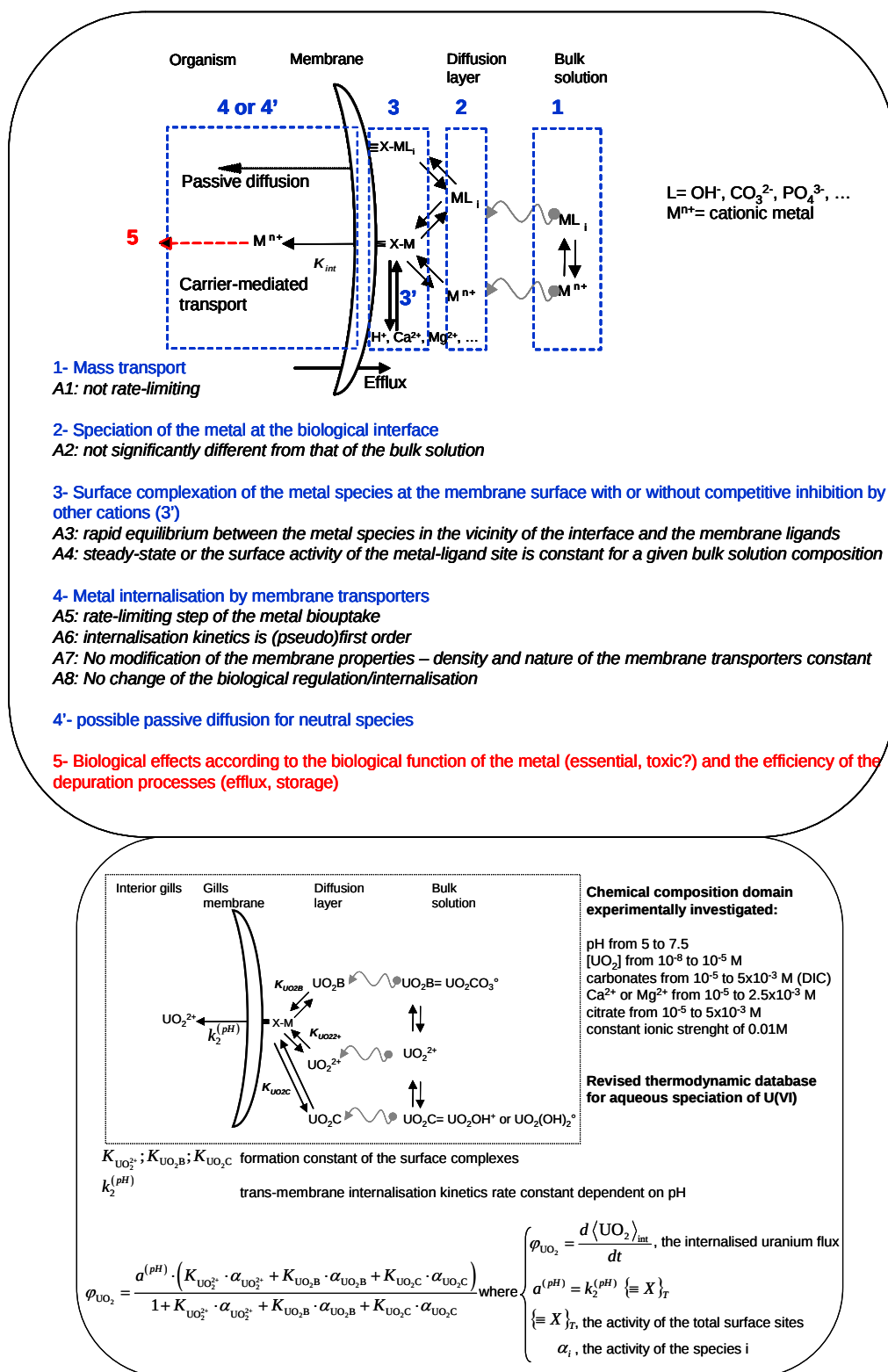
Figure 4 The main metal-cell interaction steps taken into account in the Biotic Ligand Model (BLM) and the underlying assumptions (upper image) ; and the most probable pre-equilibrium model to explain uranium-gills interactions for the investigated chemical domain.(lower image)
