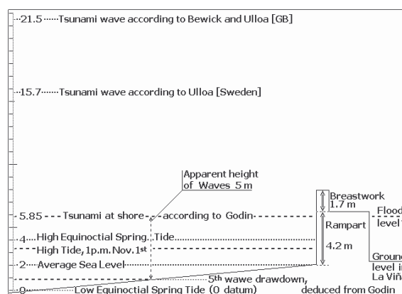
Fig. 1: Comparison of the normal scale of hydrographic levels in Cadiz (0-4 m) and the wave-setting proposed by contemporary authors. That the run-up reached the height of the rampart, but not above the breastwork, is dictated by the extent of damages and inundation. The level of the base of the town-wall comes from an excerpt of Godin's Spanish report in [8].
